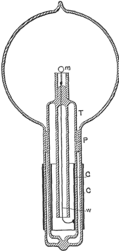
FIG. 22.—TYPE OF BULB WITHOUT LEADING-IN WIRE.
