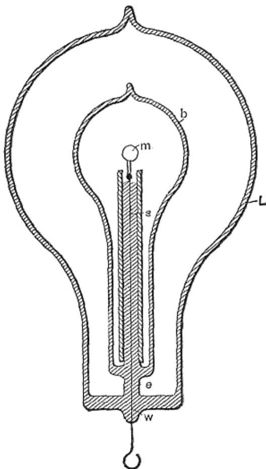
FIG. 29.—LAMP WITH INDEPENDENT AUXILIARY BULB.
