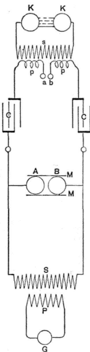
FIG. 2.—IMITATING THE SPARK OF A HOLTZ MACHINE.
