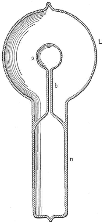
FIG. 12. BULBS FOR PRODUCING ROTATING BRUSH.
