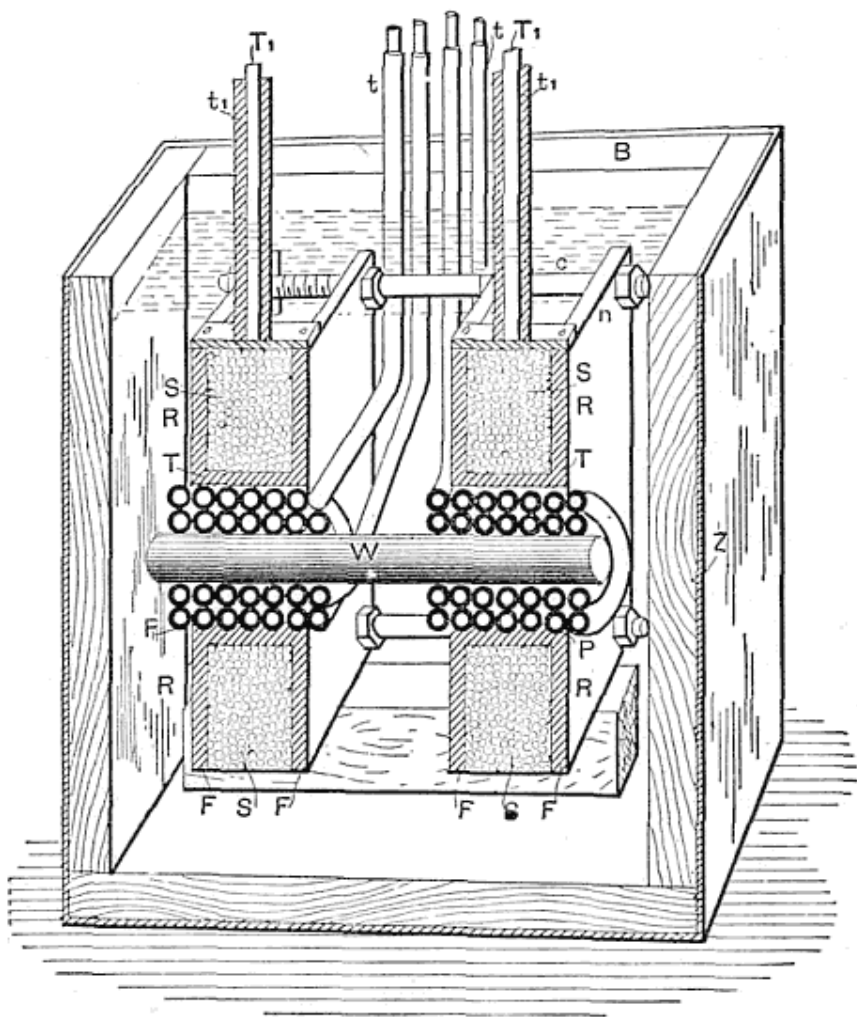
FIG. 3.—DISRUPTIVE DISCHARGE COIL.
