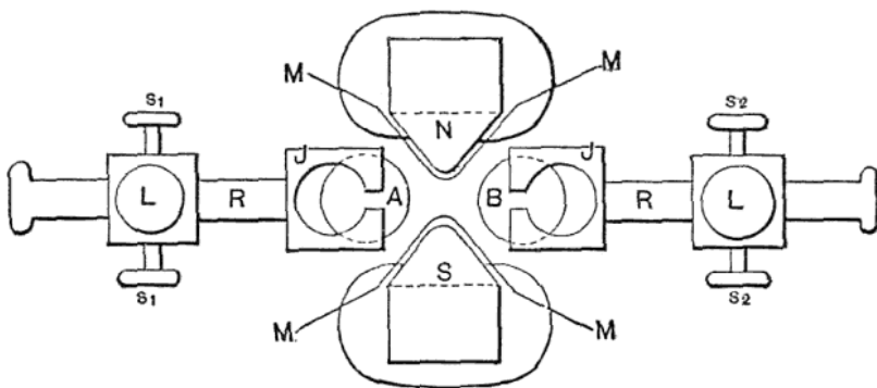
FIG. 4.—ARRANGEMENT OF IMPROVED DISCHARGER AND MAGNET.
