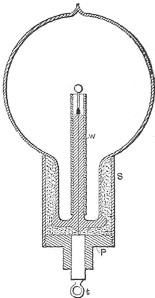
FIG. 19.—IMPROVED BULB WITH SOCKET AND SCREEN.
