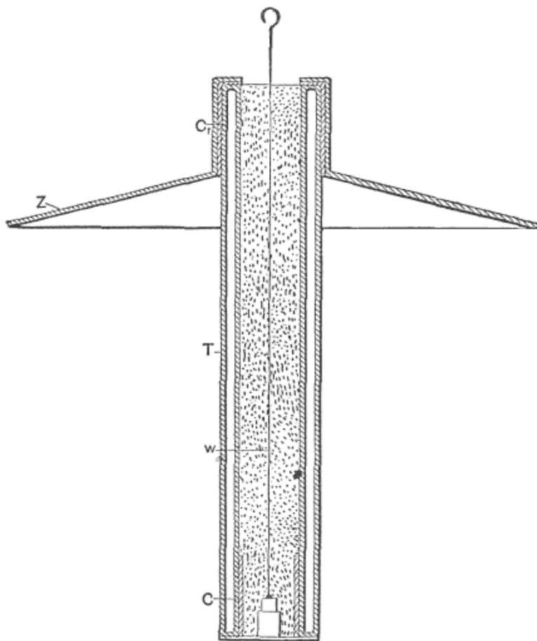
FIG. 27.—PHOSPHORESCENT TUBE WITH INTENSIFYING REFLECTOR.
