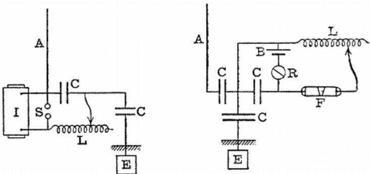
FIG. 25.—LODGE-MUIRHEAD SYNTONIC RECEIVER. I, induction coil; S, spark gap; A, aerial; CC, condensers; E, earth plate; R, relay; L, variable inductance; F, filings tube; B, battery.
