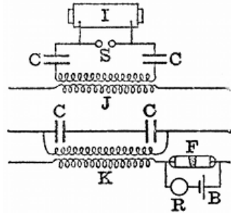
FIG. 21.—BRAUN'S NON-EARTHED RECEIVER. I, induction coil; CC, condensers; S, spark gap; J, transmitting jigger; K, receiving jigger; F, filings tube; R, relay; B, battery.
