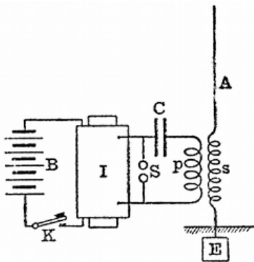
FIG. 9.—MARCONI-BRAUN SYSTEM OF INDUCING ELECTROMOTIVE FORCE IN AN AERIAL, A, B, battery; K, key; I, induction coil; S, spark gap; C, Leyden jar; E, earth plate; ps, oscillation transformer.
