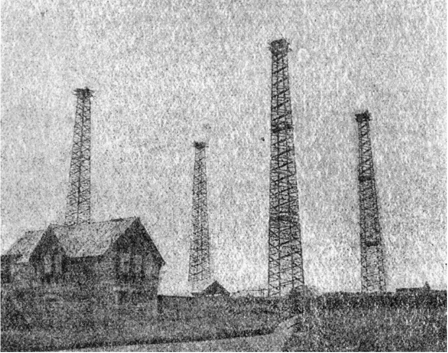
FIG. 26.—WOODEN TOWERS SUPPORTING THE MARCONI AERIAL AT POLDHU POWER STATION, CORNWALL, ENGLAND.
