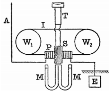
FIG. 18.—MARCONI MAGNETIC RECEIVER. W_1W_2 , wheels; I, iron wire band; P, primary coil; S, secondary coil; T, telephone; A, aerial; E, earthplate.
