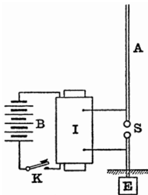
FIG. 3.—SIMPLE MARCONI RADIATOR. B, battery; I, induction coil; K, signalling key; S, spark gap; A, aerial wire; E, earth plate.
