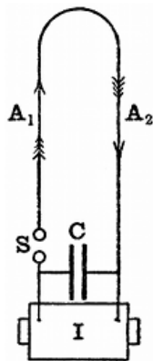
FIG. 12.—NON-RADIATIVE CLOSED LOOP AERIAL.
