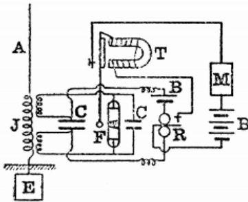
FIG. 20.—MARCONI RECEIVER. A, aerial; J, jigger; CC, condensers; F, filings tube; T, tapper; R, relay; B, battery; M, Morse printer.
