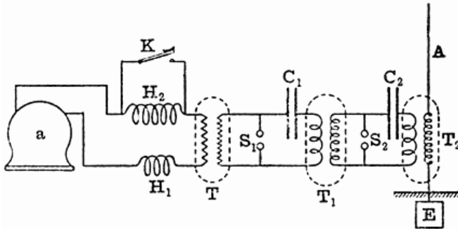
FIG. 15.—ALTERNATING-CURRENT DOUBLE-TRANSFORMATION POWER PLANT FOR GENERATING ELECTRIC WAVES (Fleming). a , alternator; H_1H_2 , choking coil; K , signalling key; T , step-up transformer; S_1S_2 spark-gap; C_1C_2 condensers; T_1T_2 , oscillation transformers; A , aerial; E , earthplate.
