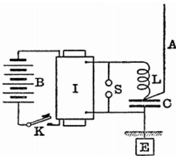
FIG. 14.—BRAUN'S RADIATOR. B, battery; I, induction coil; K, key; S, spark-gap; L, inductance coil; C, condenser; A, aerial.
