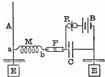
FIG. 19.—SLABY RECEIVER. A, aerial; E, earth plate; F, coherer; M, multiplier; C, condenser; R, relay; B, battery; E, earth plate.
