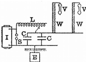
FIG. 22.—SEIBT'S APPARATUS FOR EXHIBITING ELECTRIC RESONANCE. I, induction coil; S, spark gap; CC, condensers; L, variable
