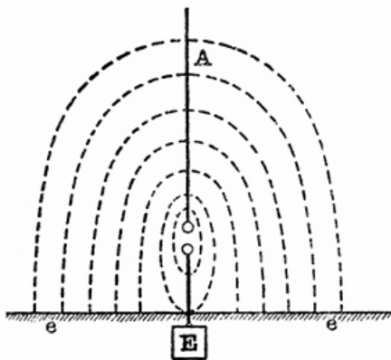
FIG. 4.—LINES OF ELECTRIC STRAIN (DOTTED LINES) EXTENDING BETWEEN A MARCONI AERIAL, A, AND THE EARTH ee BEFORE DISCHARGE.
