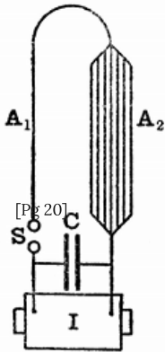
FIG. 13.—SLABY'S LOOP RADIATOR.
