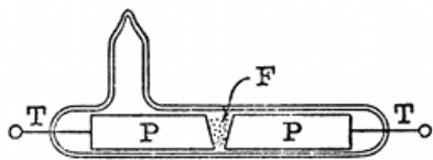
FIG. 16.—MARCONI SENSITIVE TUBE OR METALLIC FILINGS KUMASCOPE. PP, silver plugs; TT, platinum wires; F, nickel and silver filings.
