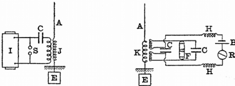
FIG. 23.—MARCONI TRANSMITTER AND RECEIVER. I, induction coil; A, aerial; E, earth plate; HH, choking coils; S, spark gap; J, transmitting jigger; K, receiving jigger; R, relay; C, condenser; F, filings tube; B, battery. Many practical details are omitted.
