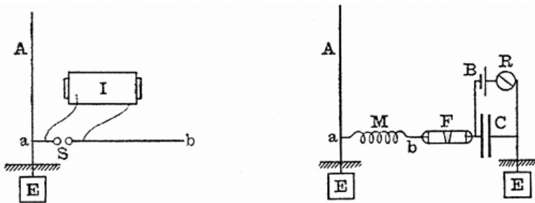
FIG. 24.—SLABY-ARCO SYNTONIC TRANSMITTER AND RECEIVER. I, induction coil; M, multiplier; B, battery; A, aerial; F, filings tube; R, relay; E, earth plate; C, condenser.
