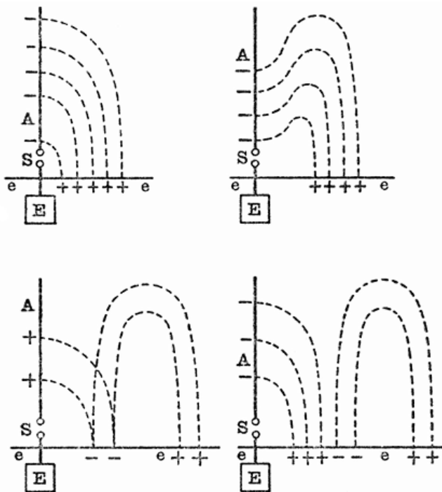
FIG. 7.—SUCCESSIVE STAGES IN THE PRODUCTION OF A SEMI-LOOP OF ELECTRIC STRAIN BY A MARCONI AERIAL RADIATOR.
